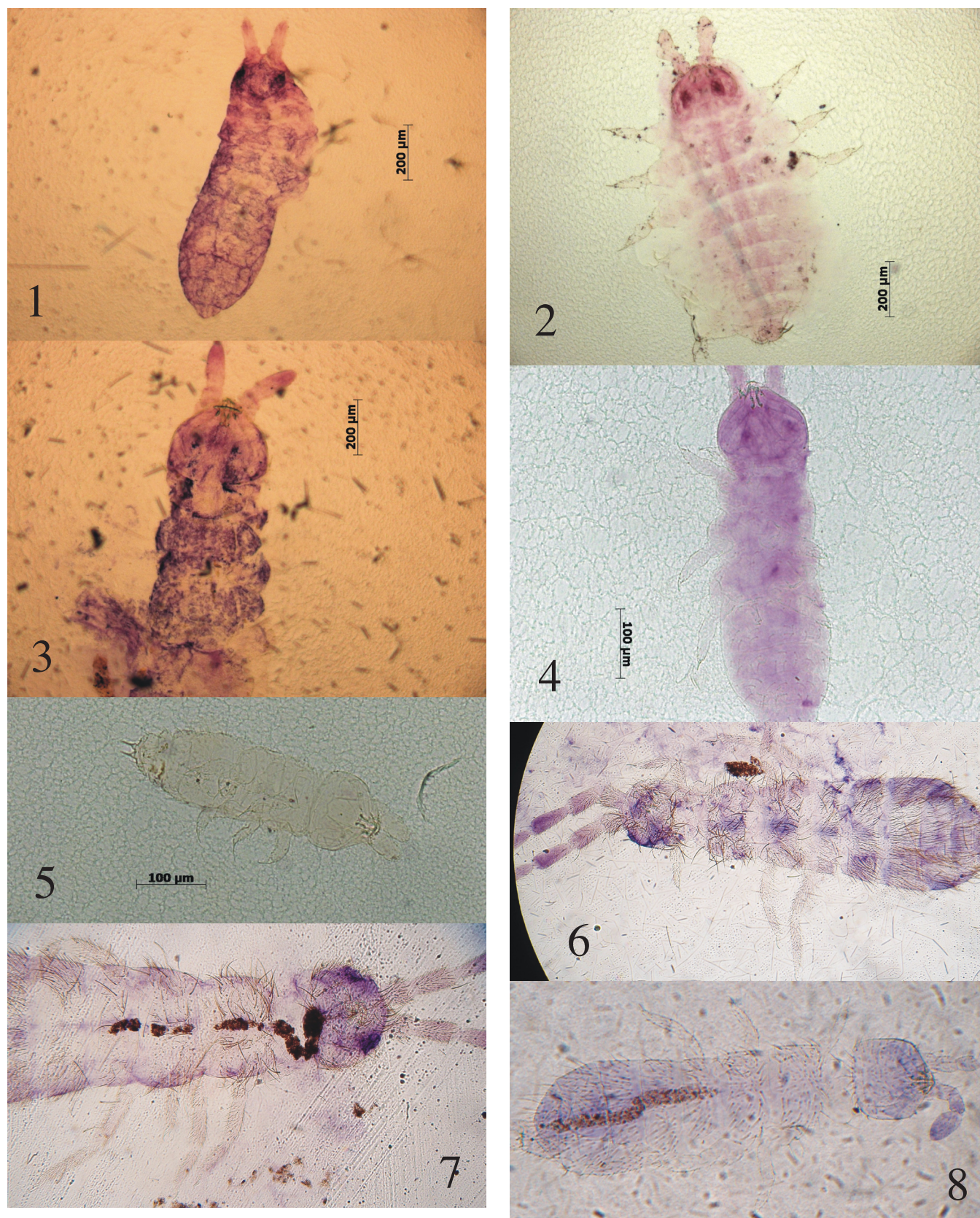
Figuras 1-8. Colémbolos del Nevado de Colima. 1. Pseudachorutes simplex Maynard. 2. Ceratophysella succinea Gisin. 3. Hypogastrura perplexa Christiansen & Bellinger. 4. Schoettella glasgowi Folsom. 5. Gnathogastrura Díaz & Najt. 6. Isotoma viridis Bourlet. 7. Isotoma delta MacGillivray. 8. Desoria flora Christiansen & Bellinger.
