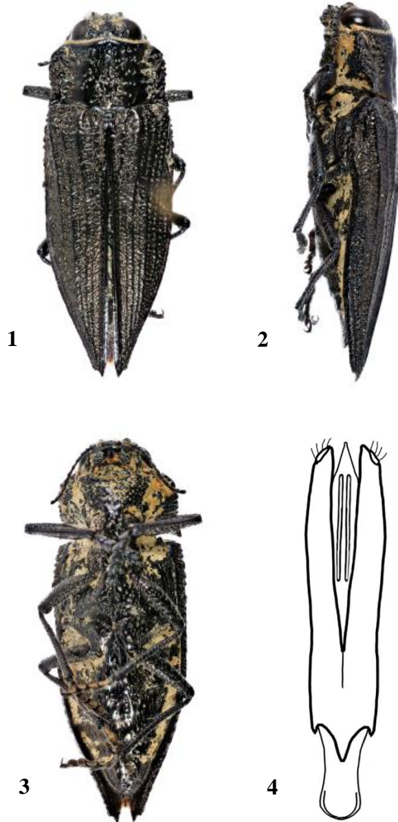
Figures 1–4. Ectinogonia toratensis , male holotype: 1) habitus, 2) lateral view, 3) ventral view, 4) aedeagus, dorsal view.
